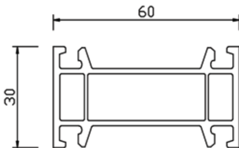
NAME :54 frame WEIGHT:0.73kg/m
