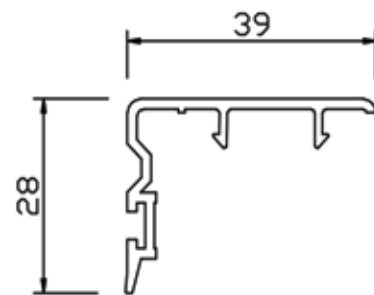
NAME :80 frame WEIGHT:1.13kg/m
