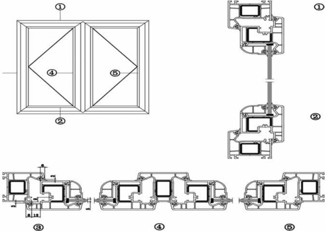
60 casement assembly drawing
