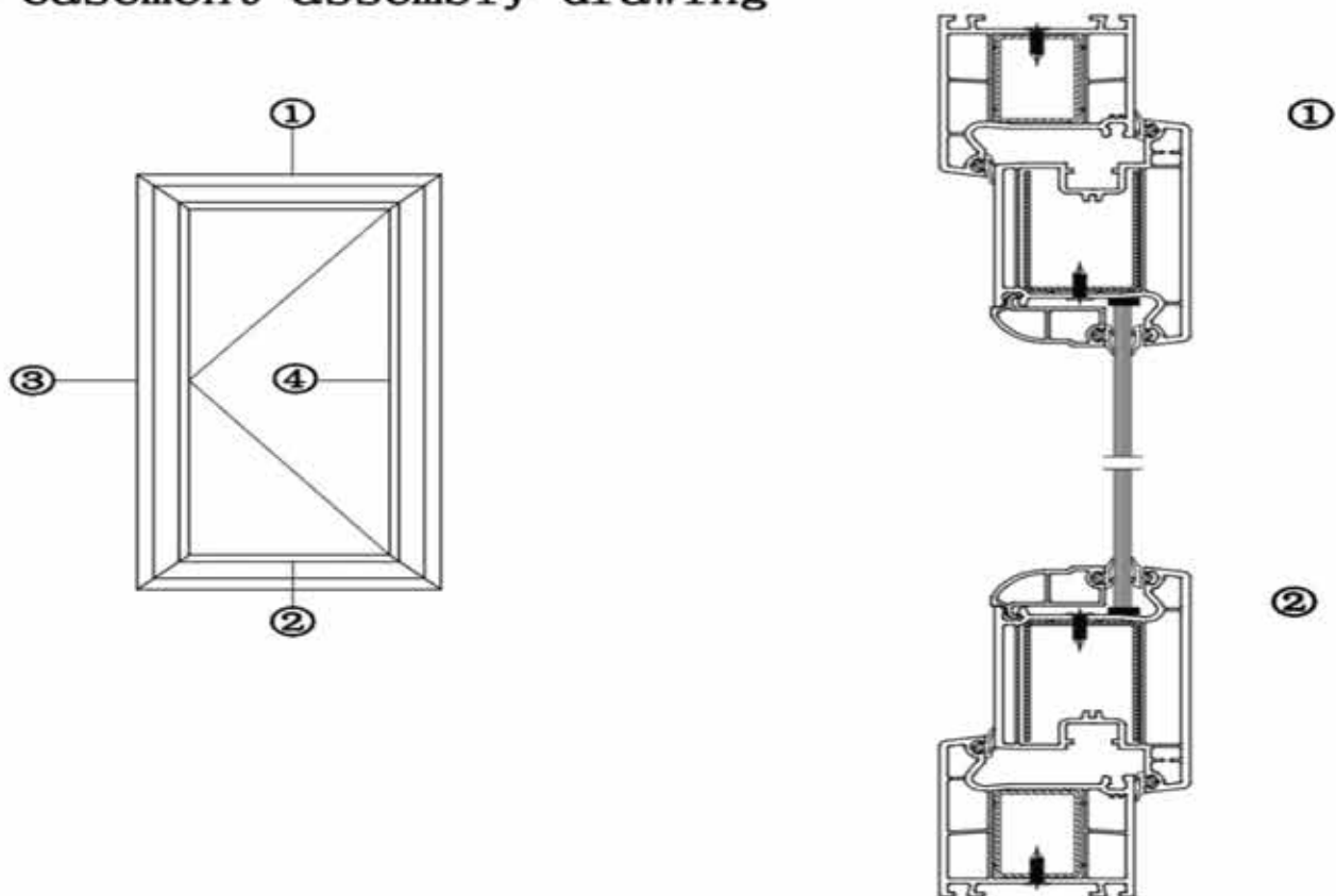
60 casement assembly drawing
