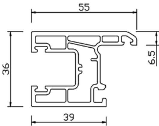
NAME :54 frame WEIGHT:0.73kg/m
